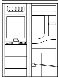
Details: Interior door panelling and quarter-section timbering
